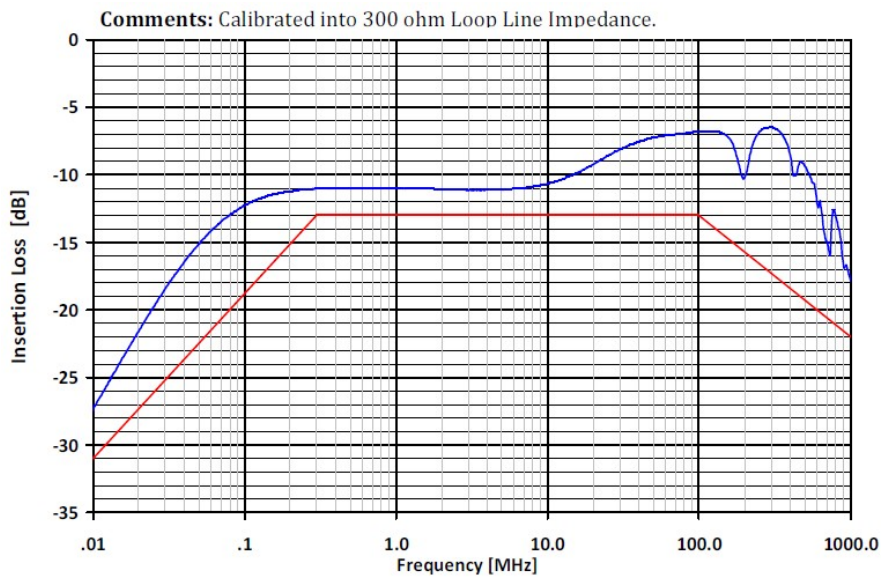
典型插入损耗
