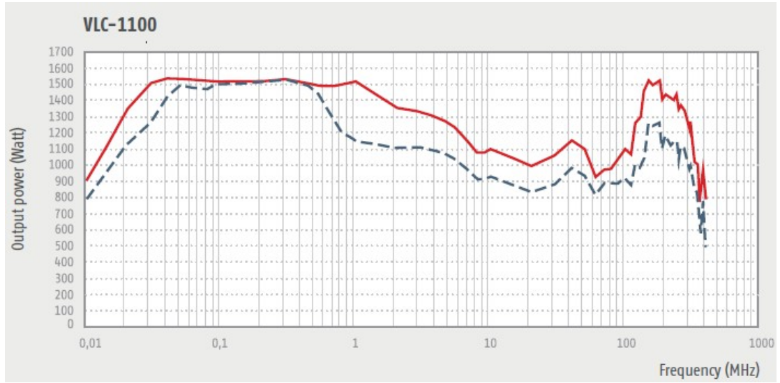
VLC-1100----- 1dB/— 3dB 压缩点输出功率
