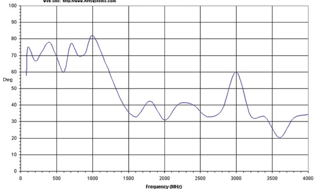
Half Power Beamwidth Model SAS-517
