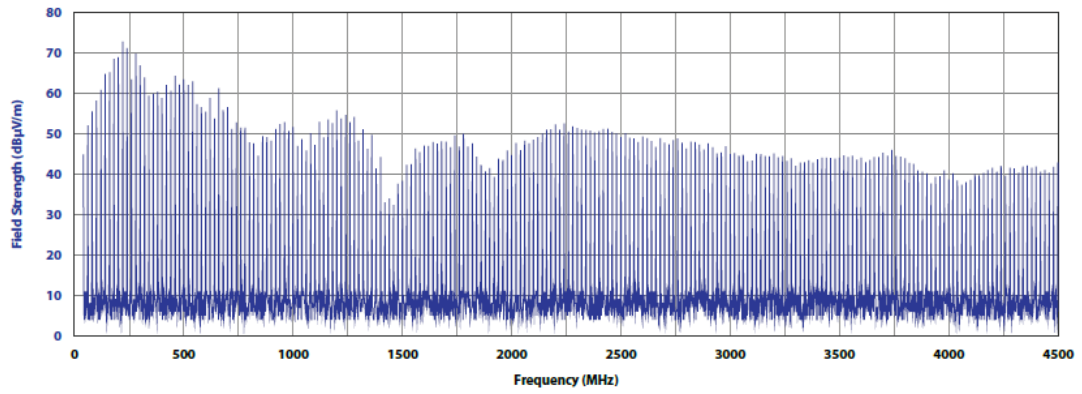
Typical Radiated Output at 3-meter Distance (Antenna Height Fixed at 1 meter)
