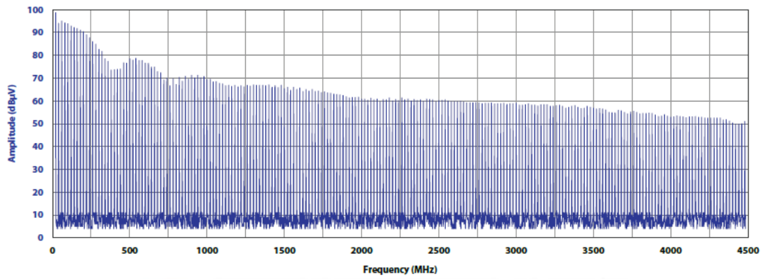
Typical Direct (Conducted) Output
