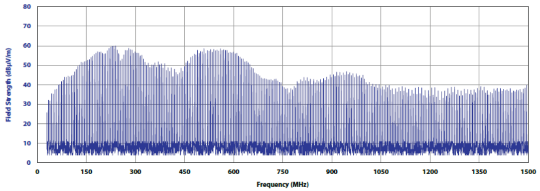
Typical Radiated Output at 3-meter Distance (Antenna Height Fixed at 1 meter)
