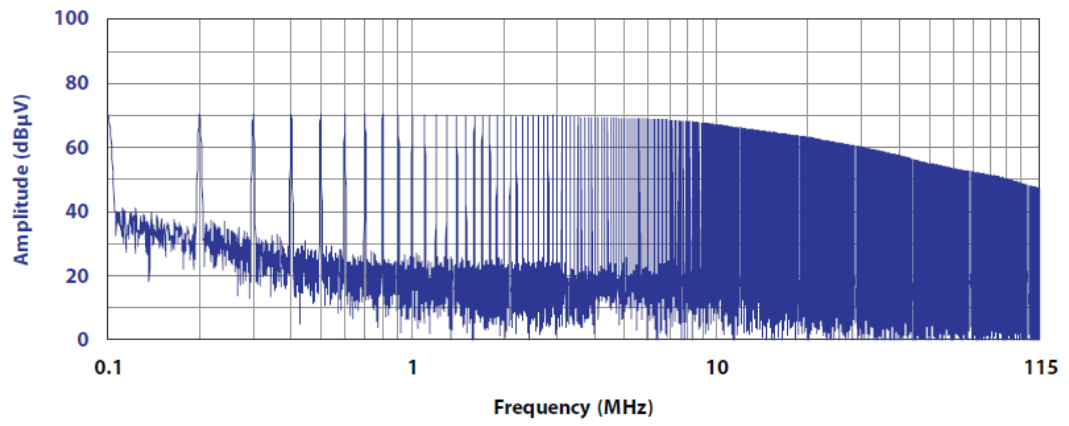
Typical Output - 100 kHz Step Size
