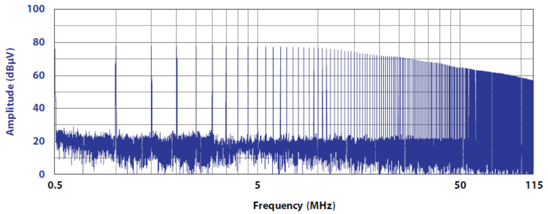
Typical Output - 500 kHz Step Size
