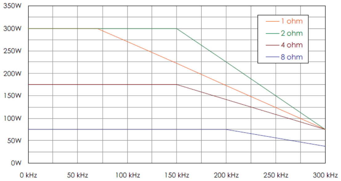
ARI-300K Minimum Power Output Specifications
