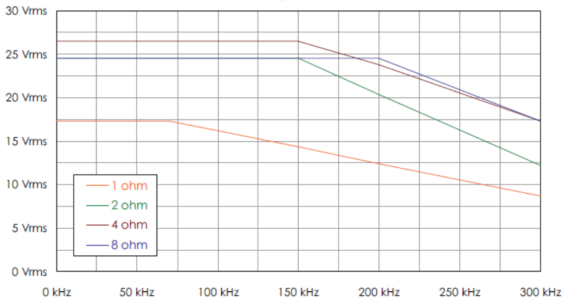
ARI-300K Minimum Voltage Output Specifications
